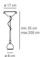
Fenice 8 with tranformer HALO max 1x50W/12V (GY 6,35) - QT 12
