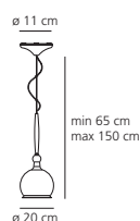
Fenice 20 HALO max 1x150W (B 15d) - ECO, dimmable
