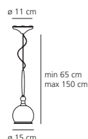
Fenice 15 HALO max 1x70W (B 15d) - ECO, dimmable
