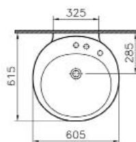
Wall-hung washbasin, 60 cm (with integrated trap cover)
