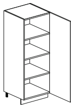
1 anta, ripiani l 300, 450, 600 1 door, shelves w 11 13/16", 17 11/16", 23 5/8"
