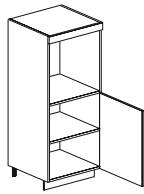
anta, ripiani, vano forno l 600 door, shelves, oven unit w 23 5/8"
