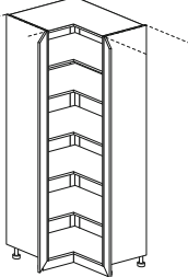
p 950 - angolare, 2 ante apertura 180°, ripiani l 950 d 23 5/8" - corner, 2 doors with 180° opening, shelves w 37 1/2"
