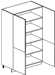
ante divise, ripiani l 900, 1200 divided doors, shelves w 35 7/16", 47 1/4"
