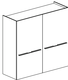
h 1980-2100-2200 - p 700 ante scorrevoli complanari l 1800 h 77 15/16"-82 11/16"-87 3/8" - d 27 9/16" sliding co-planar doors w 70 7/8"
