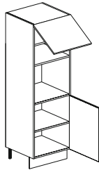
h 1860-1980 - anta, anta a ribalta, ripiani, vano forno l 600 h 73 1/4"-77 15/16" - door, flap opening, shelves, oven unit w 23 5/8"
