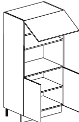
h 1860-1980 - ante, anta a ribalta, ripiani, vano forno l 900; l 762 escluso h 1860 h 73 1/4"-77 15/16" - doors, flap opening, shelves, oven unit w 35 7/16"; w 30" exc h 73 1/4"
