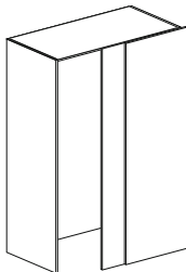
h 1860-1980 p 720 - angolo ripostiglio, 1 anta scorrevole e 1 fissa l 1330 h 73 1/4"-77 15/16" p 28 3/8" - closet corner, 1 sliding door and 1 fixed door w 52 3/8"
