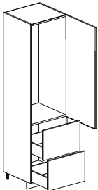
h 1980-2100-2220 - anta, 2 estraattori, vano frigo l 600 h 77 15/16"-82 11/16"-87 3/8" door, 2 pullers, refrigerator unit w 23 5/8"
