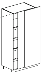
p 600 - angolo, 1 anta scorrevole e 1 fissa, ripiani l 1250, 1287, 1350 d 23 5/8" - corner, 1 sliding door and 1 fixed door, shelves w 49 3/16", 50 11/16", 53 1/8"
