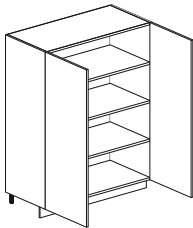
2 ante, ripiani l 900, 1200 2 doors, shelves w 35 7/16", 47 1/4"
