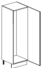
1 anta, vano frigo l 600 h 1380 solo questa colonna 1 door, refrigerator unit w 23 5/8" h 54 5/16" only this tall unit
