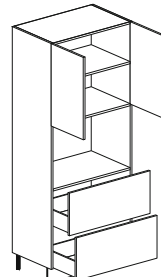
ante, 2 estraattori, ripiani, vano forno l 900; l 762 escluso h 1860 doors, 2 pullers, shelves, oven unit w 35 7/16"; w 30" exc h 73 1/4"
