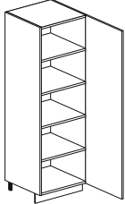
1 anta, ripiani l 300, 450, 600 1 door, shelves w 11 13/16", 17 11/16", 23 5/8"
