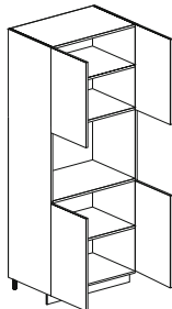
ante, ripiani, vano forno l 900; l 762 escluso h 1860 doors, shelves, oven unit w 35 7/16"; w 30" exc h 73 1/4"
