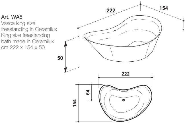
VASCA KING SIZE IN CERAMILUX KING SIZE BATHTUB IN CERAMILUX
