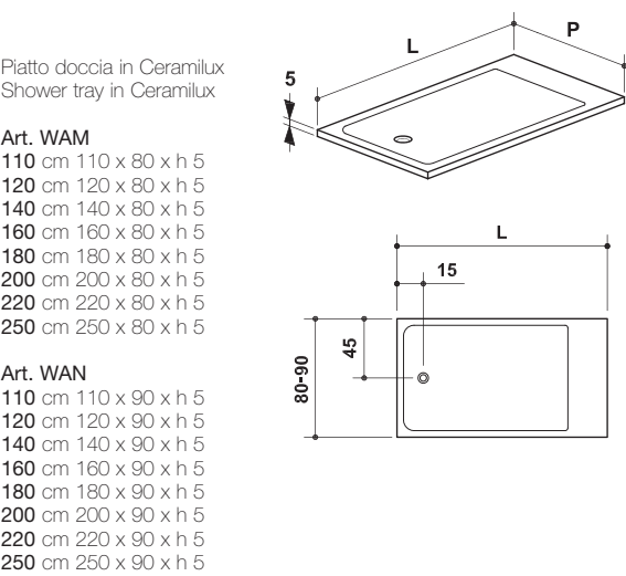
PIANI DOCCIA IN CERAMILUX SHOWER TRAY IN CERAMILUX
