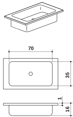
LAVABO A FILO PIANO IN CERAMILUX FLUSH WASHBASIN IN CERAMILUX
