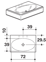
Art. D4B Piano lavabo monoblocco Washbasin console cm 78 x 52 x h 15
