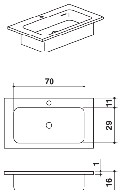
LAVABO A FILO PIANO IN CERAMILUX FLUSH WASHBASIN IN CERAMILUX
