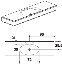
Art. D4I Piano lavabo monoblocco Washbasin console cm 180 x 52 x h 15
