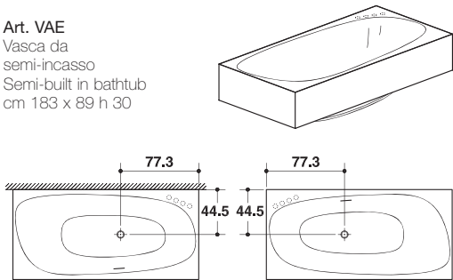
VASCA DA SEMINCASSO IN CRISTALPLANT SEMI BUILT-IN BATHTUB IN CRISTALPLANT
