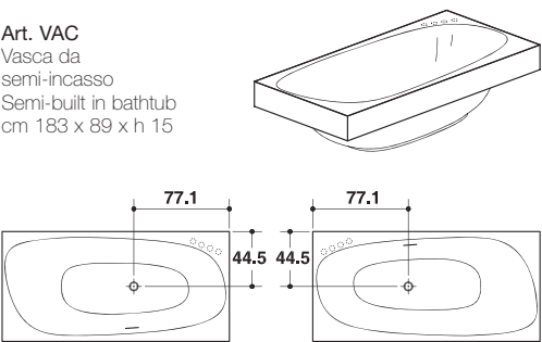
VASCA DA SEMINCASSO IN CRISTALPLANT SEMI BUILT-IN BATHTUB IN CRISTALPLANT
