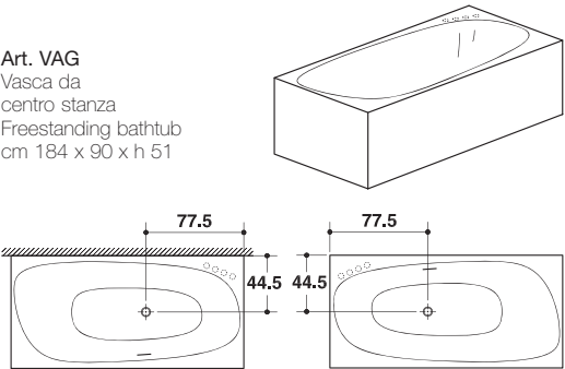
VASCA FREESTANDING IN CRISTALPLANT FREESTANDING BATHTUB IN CRISTALPLANT
