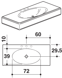
Art. D4I Piano lavabo monoblocco Washbasin console cm 180 x 52 x h 15
