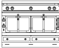
CHÂTEAU 120 2 vaulted ovens of 55L (gas or electric / all electric) W. 120cm, D. 70cm, H. 92cm
