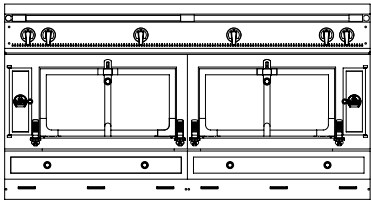
GRAND PALAIS 180 2 large vaulted ovens of 74L ( gas and electric / all electric) W. 180cm, D. 70cm, H. 92cm
