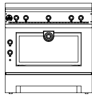
GRAND MAMAN 90 1 large vaulted oven of 74L (gas or electric) W. 90cm, D. 70cm, H. 90cm
