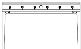
INDUCTION TABLE Wall or central position 4 induction plates W. 150cm, D. 70cm, H. 92cm
