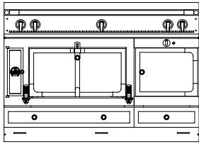
GRAND CHÂTELET 135 1 large vaulted oven of 74L (gas or electric). Warming cupboard on the right W. 135cm, D. 70cm, H. 92cm
