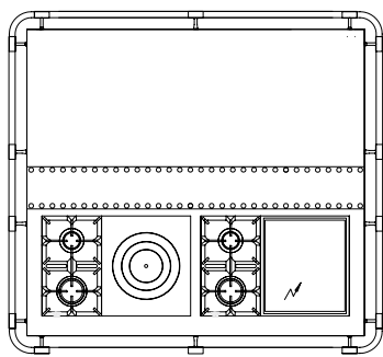
CHÂTEAU 150 ISLAND UNIT W. 176cm, D. 162cm, H. 92cm
