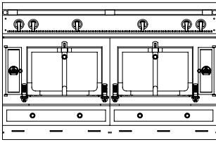
CHÂTEAU 150 2 vaulted ovens of 55L ( gas and electric / all electric) W. 150cm, D. 70cm, H. 92cm
