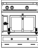
CASTEL 75 1 large vaulted oven of 55L (gas or electric) W. 75cm, D. 70cm, H. 92cm.
