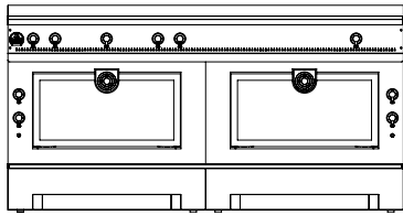
GRAND PAPA 180 2 large vaulted ovens of 74L ( gas and electric / all electric) W. 180cm, D. 70cm, H. 90cm
