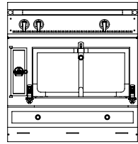
GRAND CASTEL 90 1 large vaulted oven of 74L (gas or electric) W. 90cm, D. 70cm, H. 92cm
