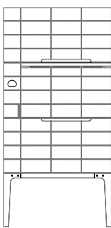
OVEN TOWER Electric vaulted oven (74L) W. 90cm, D. 70cm, H. 184cm
