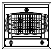
FLAMBERGE ROTISSERIE GAS Available in the same colours and trims as the Châteaux range. W. 81,5cm, D. 38cm, H. 79,2cm
