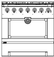
LA CORNUE 1908 Large vaulted oven gas or electric with an electric grill. Gas cooktop. Storage drawer in the lower part. W. 90cm, D. 70cm, H. 90cm
