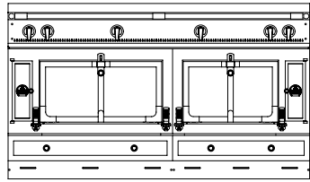
CHÂTEAU 165 1 large vaulted oven of 74L (gas or electric) and 1 vaulted oven of 55L (electric) W. 165cm, D. 70cm, H. 92cm
