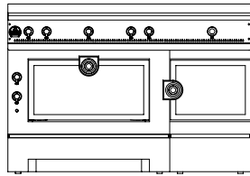
GRAND PAPA 135 1 large vaulted oven of 74L (gas or electric). Warming cupboard on the right W. 135cm, D. 70cm, H. 90cm
