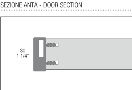
battente - leaf door
