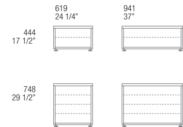
STRUTTURE CASSETTIERA SU RUOTE PER CASSETTI O VASSOI CHEST OF DRAWERS STRUCTURES ON CASTORS FOR DRAWERS OR TRAYS
