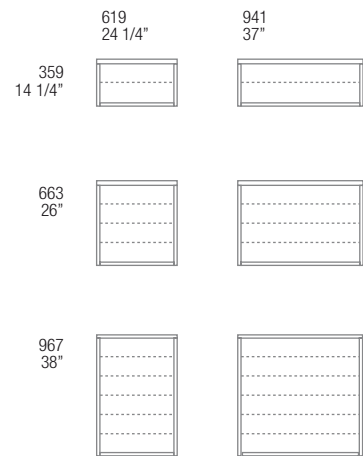
STRUTTURE CASSETTIERA A TERRA PER CASSETTI O VASSOI FREESTANDING CHEST OF DRAWERS STRUCTURES FOR DRAWERS OR TRAYS
